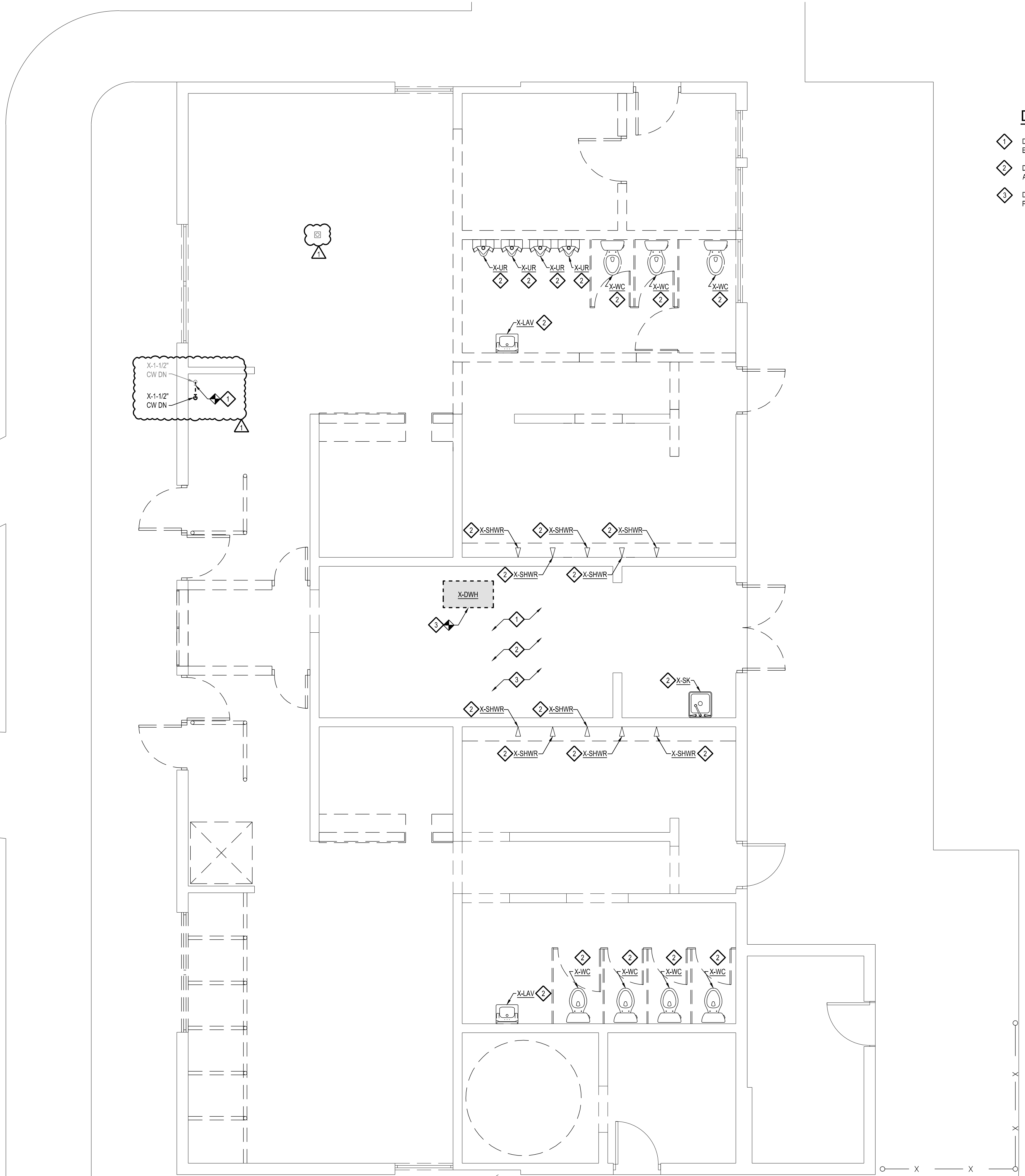
FLOOR PLAN - PLUMBING DEMOLITION SCALE: 1/4" = 1'-0"
