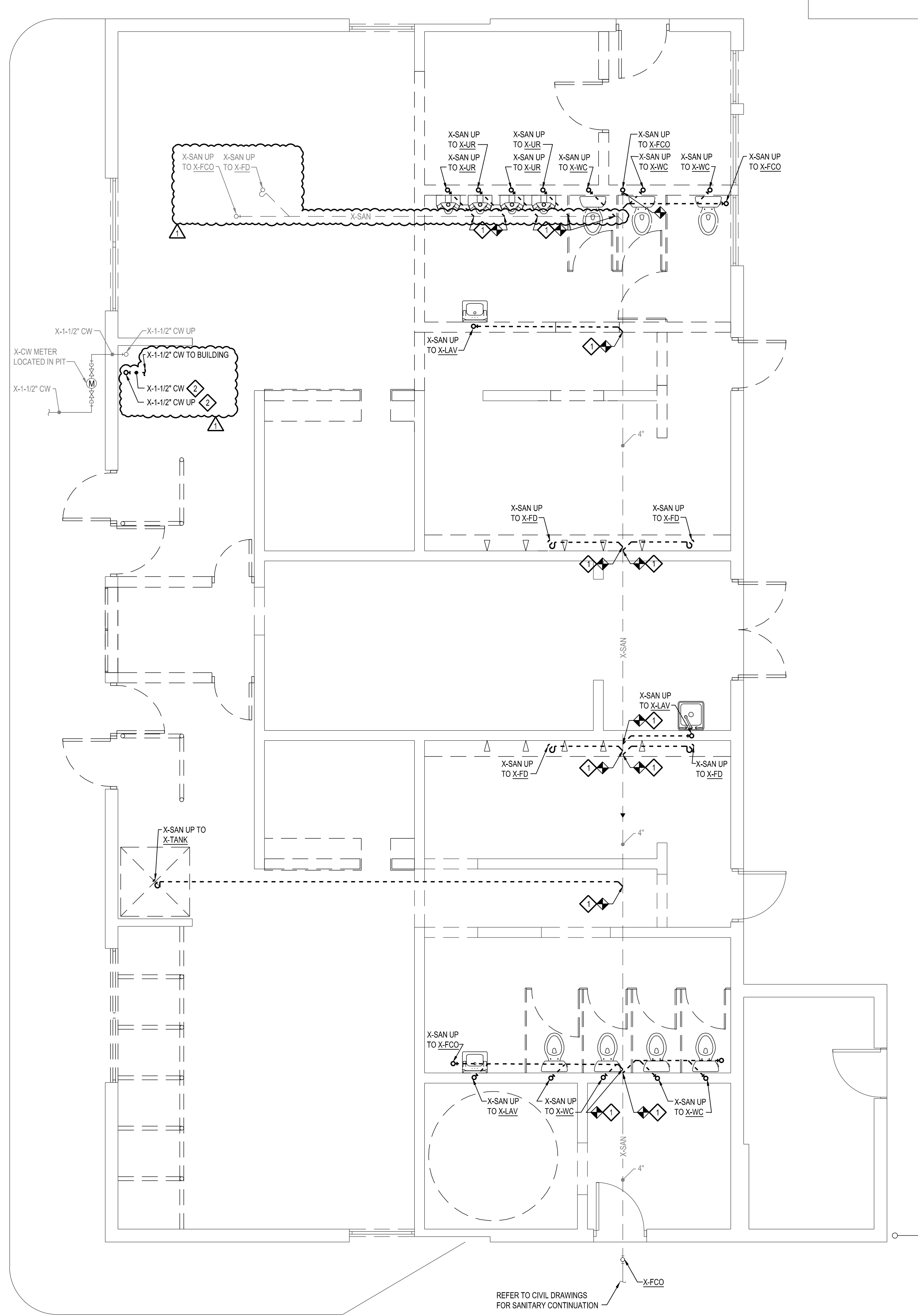
BELOW FLOOR PLAN - PLUMBING DEMOLITION SCALE: 1/4" = 1'-0"
