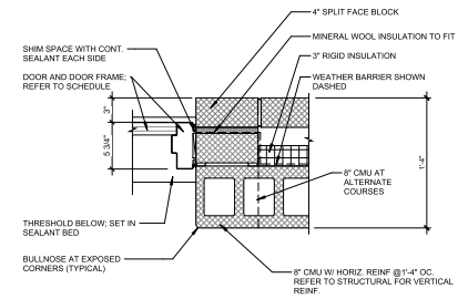
J1 TYP. JAMB DETAIL SCALE: 1 1/2" = 1'-0"
