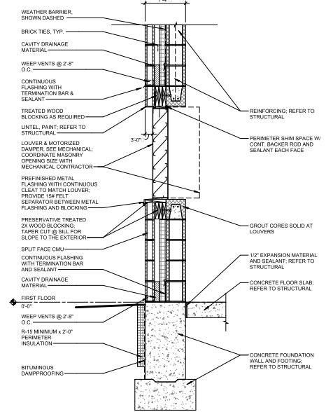
1 TYP. WALL DETAIL SCALE: 3/4" = 1'-0"
