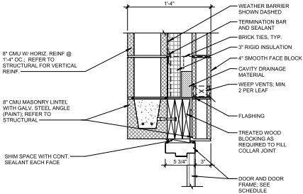
H1 TYP. HEAD DETAIL SCALE: 1 1/2" = 1'-0"
